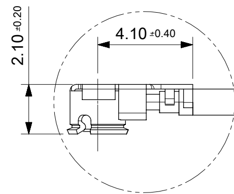
DETAIL A SCALE 6:1 CONNECTOR
