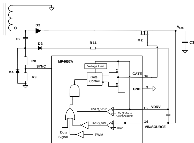
Figure 2: MP4657A Gate Driver and Start Up
