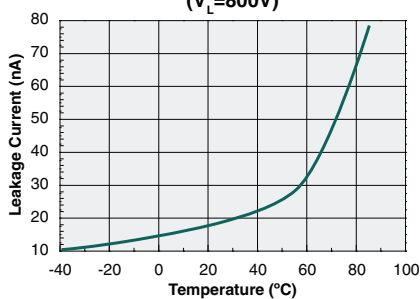
Typical Leakage Current vs. Temperature ( V_L=800\text{V} )
