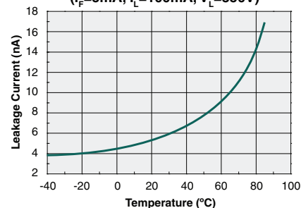
Typical Leakage Current vs. Temperature ( I_F=5\text{mA} , I_L=100\text{mA} , V_L=350\text{V} )
