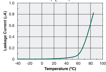
Leakage Current vs. Temperature Across Pins 5&6, 7&8 ( V_L=60\text{V} )
