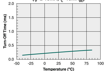
Typical Turn-Off Time vs. Temperature ( I_F=2\text{--}10\text{mA} , I_L=10\text{mA}_{\text{DC}} )
