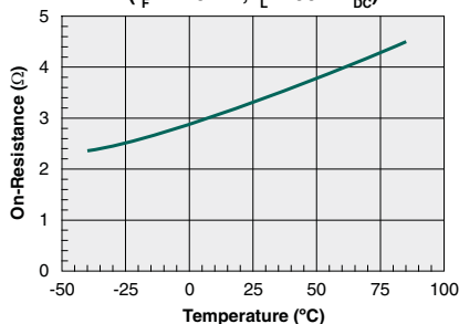
On-Resistance vs. Temperature DC-Only Configuration ( I_F=2\text{--}10\text{mA} , I_L=100\text{mA}_{\text{DC}} )
