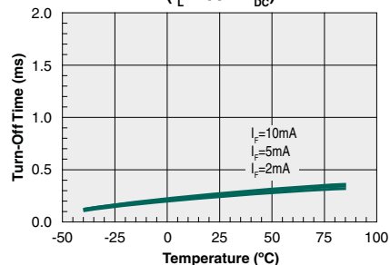
Typical Turn-Off Time vs. Temperature ( I_L=100\text{mA}_{\text{DC}} )
