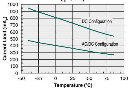
Typical Current Limit vs. Temperature ( I_F=5\text{mA} )
