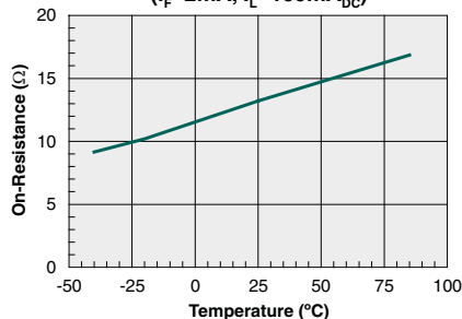
On-Resistance vs. Temperature DC-Only Configuration ( I_F=2\text{--}10\text{mA} , I_L=100\text{mA}_{\text{DC}} )
