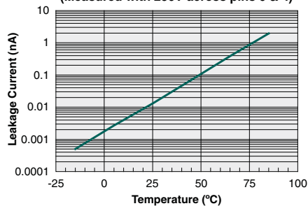
Typical Leakage Current vs. Temperature (Measured with 250V across pins 6 & 4)
