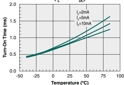
Typical Turn-On Time vs. Temperature ( I_L=10\text{mA}_{\text{DC}} )
