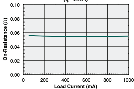
Typical On-Resistance vs. Load Current ( I_F=0\text{mA} )
