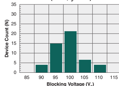
Typical Blocking Voltage Distribution (N=50, I_F=1\text{mA} )
