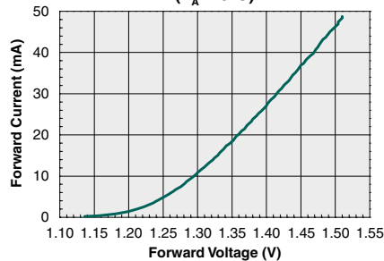
Typical LED Forward Voltage vs. Forward Current ( T_A=25^\circ\text{C} )
