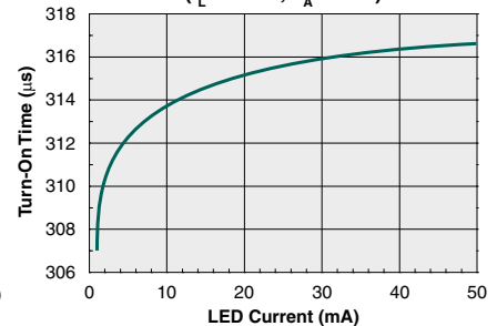
Typical Turn-On Time vs. LED Forward Current ( I_L=60\text{mA} , T_A=25^\circ\text{C} )
