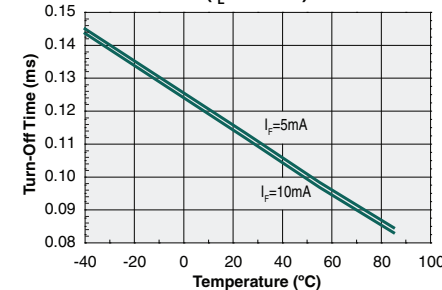
Turn-Off Time vs. Temperature ( I_L=100\text{mA} )
