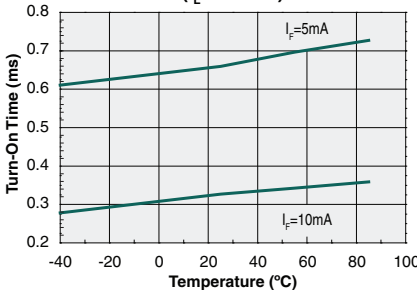
Turn-On Time vs. Temperature ( I_L=100\text{mA} )
