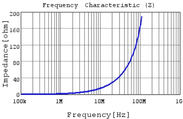
DFE18SANR24MG0 |Z|
