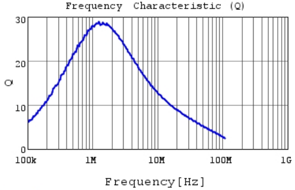
DFE18SANR24MG0 Q
