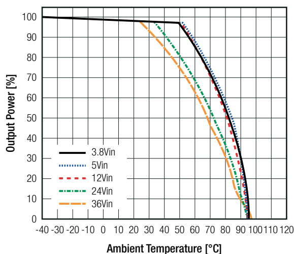
Thermal Derating
