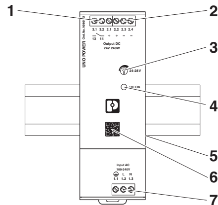
Figure 3 Location of functional elements and device connections
