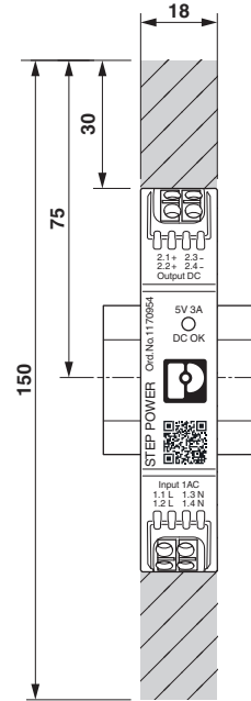
Figure 9 Device dimensions and minimum keep-out areas (in mm)
