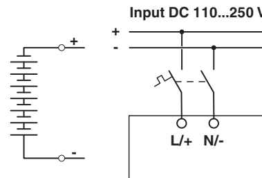
Figure 15 Pin assignment for DC supply voltage
