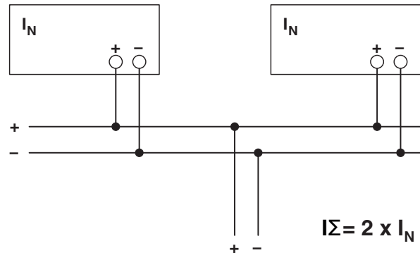
Figure 47 Schematic diagram of increased performance
