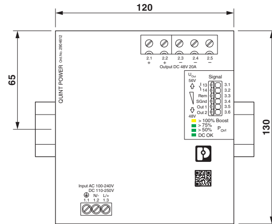
Figure 5 Device dimensions (dimensions in mm)
