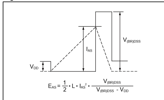
Fig.3-2 Avalanche Waveform
