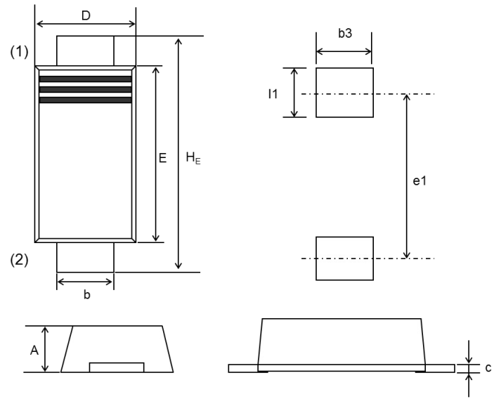
SOD-123FL, (FMDU)
