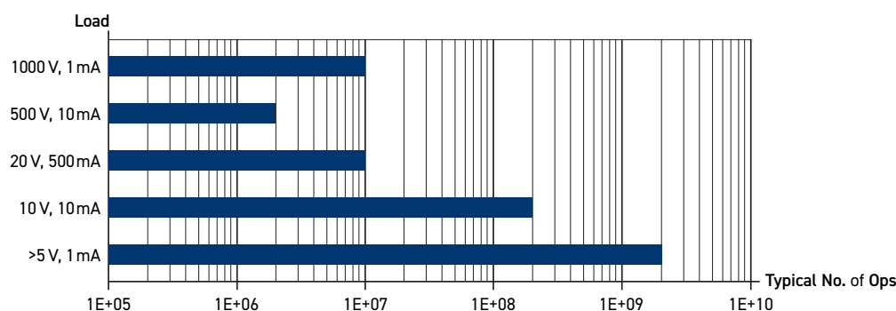
Series 119 Life Test Data
