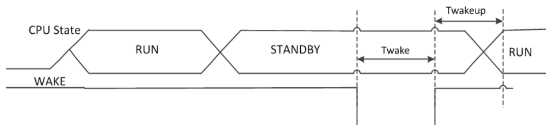
Figure 8-3 Wake Timing
