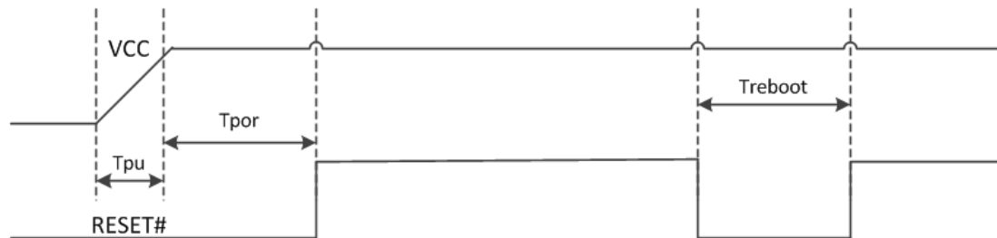
Figure 8-1 Reset Timing
