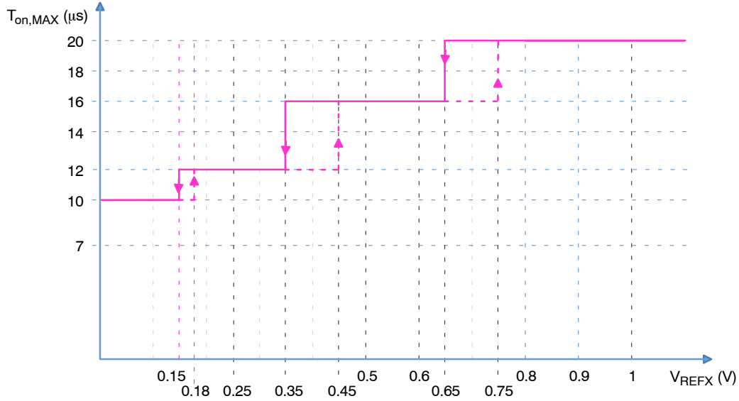
Figure 72. Variable Maximum On-time, 20- \mu s Option
