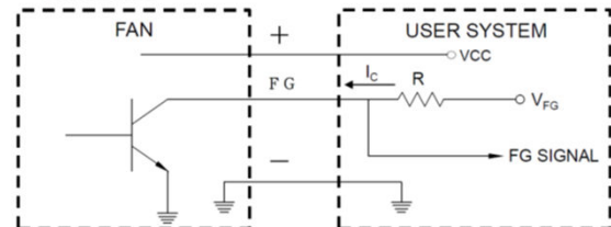
FREQUENCY GENERATOR (FG) SIGNAL
