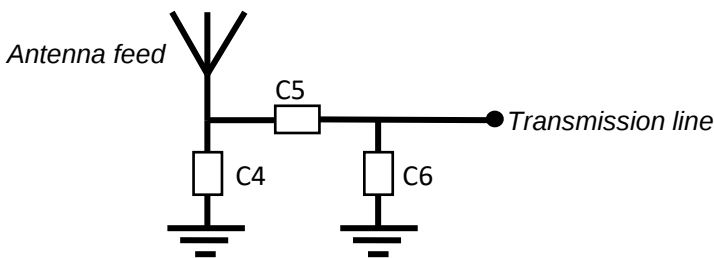
Matching circuit
