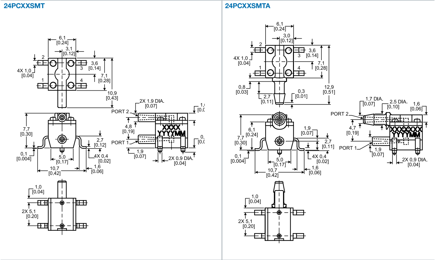
Figure 3. Mounting Dimensions (For reference only: mm/[in.])
