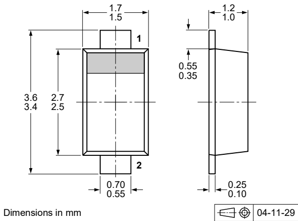
Fig. 11. Package outline SOD123F
