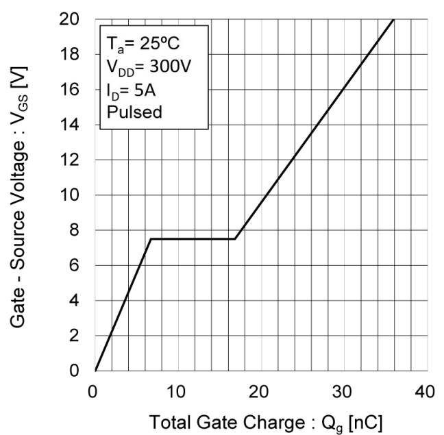
Fig.16 Gate charge
