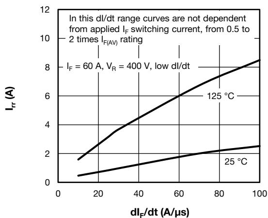
Fig. 12 - Typical Reverse Recovery Current vs. di/dt
