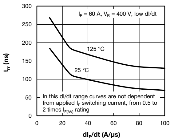
Fig. 10 - Typical Reverse Recovery Time vs. di/dt
