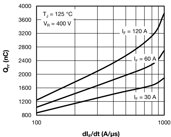
Fig. 8 - Typical Reverse Recovery Charge vs. di/dt
