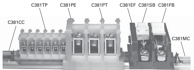
A Typical Mixture of Control Circuit Blocks, Power Blocks, Switch and Fuse Blocks in a Mounting Channel
