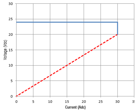
PQU650M-24P; Constant Current OCP
