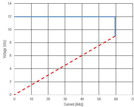
PQU650M-12P; Constant Current OCP
