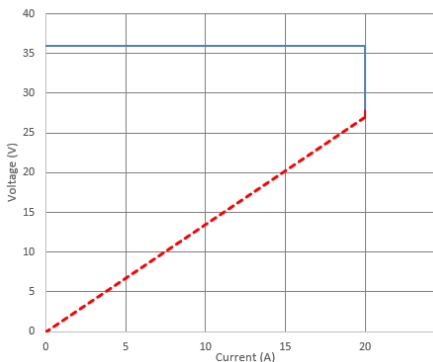
PQU650M-36P; Constant Current OCP
