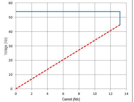
PQU650M-54P; Constant Current OCP
