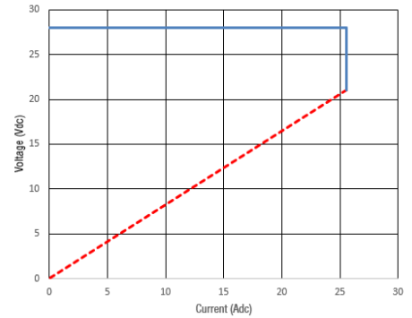
PQU650M-28P; Constant Current OCP
