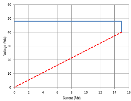
PQU650M-48P; Constant Current OCP
