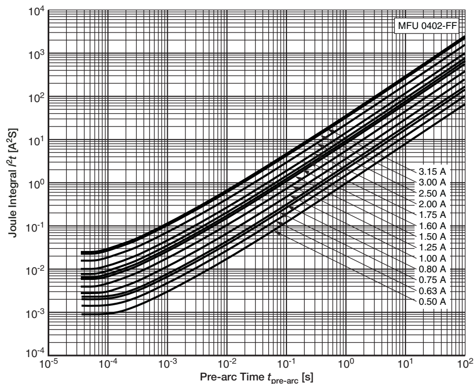
Typical I^2 t vs. t_{pre-arc} characteristic of MFU 0402 (1)
