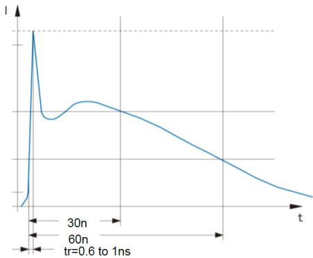
IEC61000-4-2 Waveform
