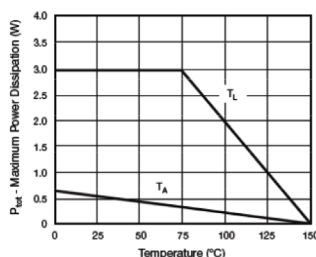
Fig. 1 - Steady State Power Duting
