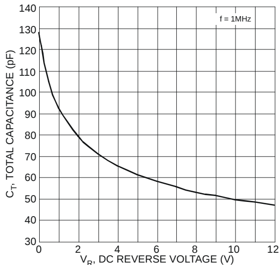
Figure 4 Typical Capacitance
