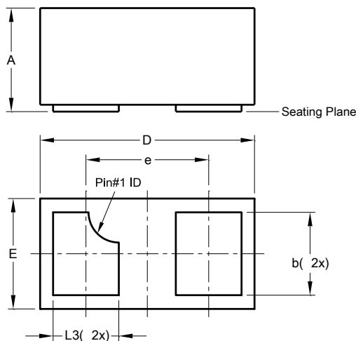
X2-DFN0603-2
