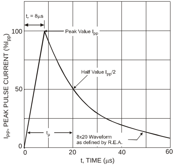
Figure 3 Typical 8 × 20μs Pulse Waveform
