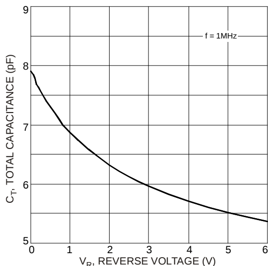
Figure 2 Typical Total Capacitance vs. Reverse Voltage
