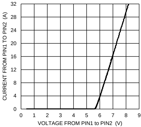
Figure 5 Pin1 to Pin2 TLP Curve ( t_p = 100\text{ns} )
