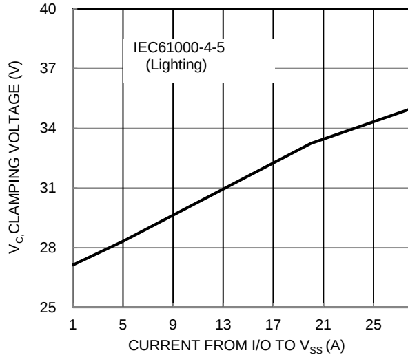
Figure 1 Clamping Voltage Characteristic
