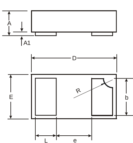
X1-DFN1006-2
