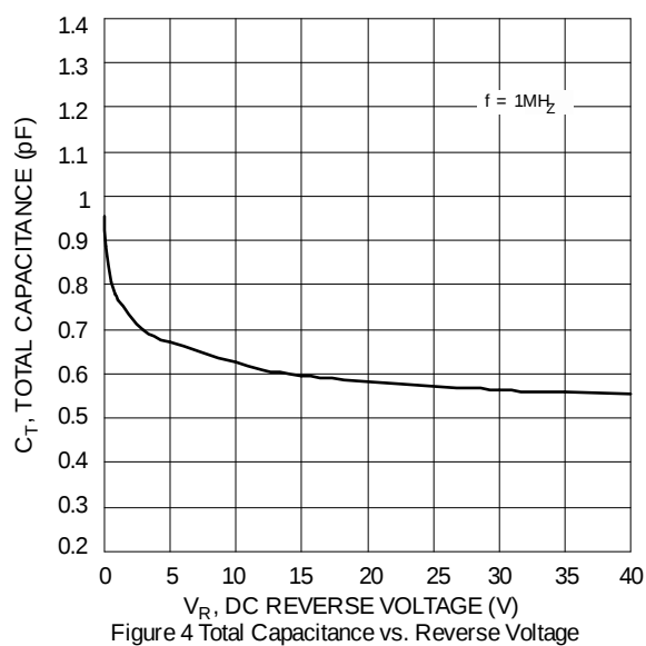
Figure 4 Total Capacitance vs. Reverse Voltage
