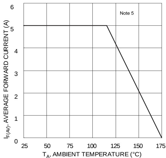
Figure 4 Forward Current Derating
