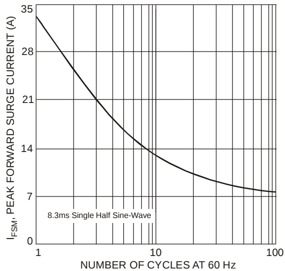
Figure 4 Maximum Non-Repetitive Peak Forward Surge Current
