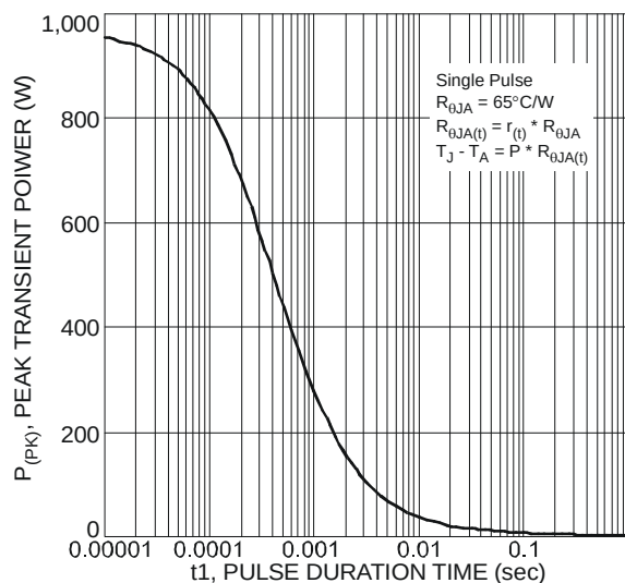
Figure 8 Single Pulse Maximum Power Dissipation
