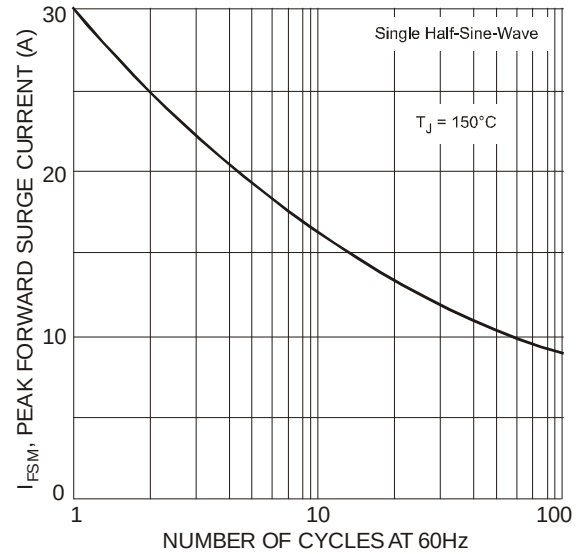
Fig. 4 Forward Surge Current Derating Curve
