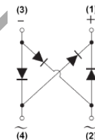
Internal Schematic
