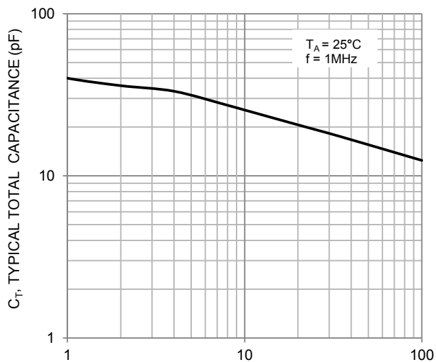
V_R , REVERSE VOLTAGE (V) Figure 4. Typical Total Capacitance (Per Leg)
