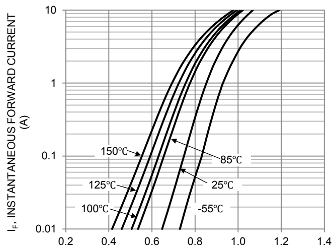
V_F , INSTANTANEOUS FORWARD VOLTAGE (V) Figure 2. Typical Forward Characteristics (Per Leg)
