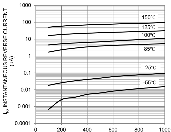
V_R , REVERSE VOLTAGE (V) Figure 5. Typical Reverse Characteristics
