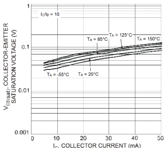
Fig. 20 Typical V_{CE(sat)} vs. I_C
