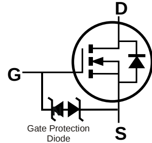
Equivalent Circuit per Element
